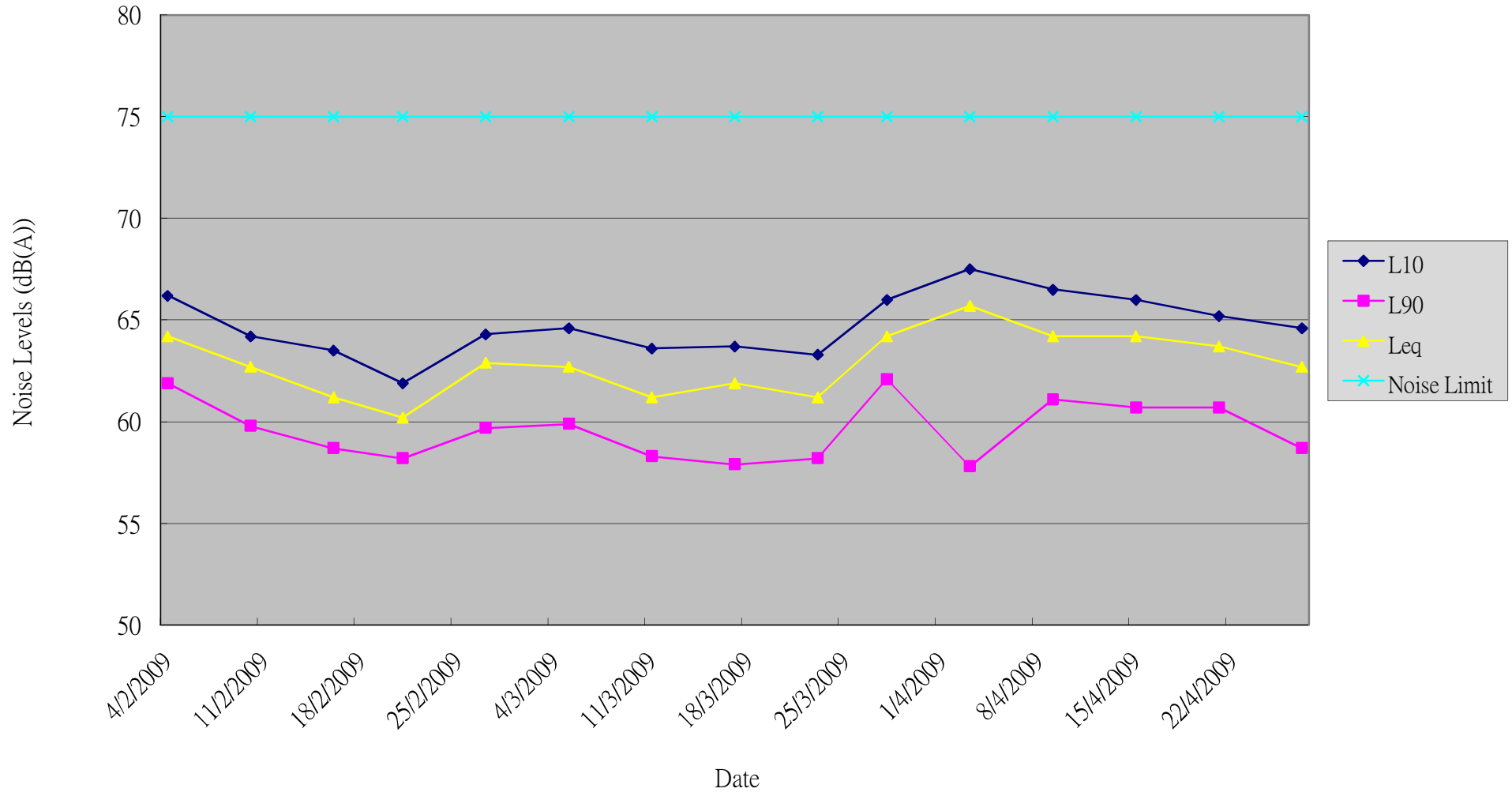
Noise Monitoring Record (February 2009 - April 2009)
